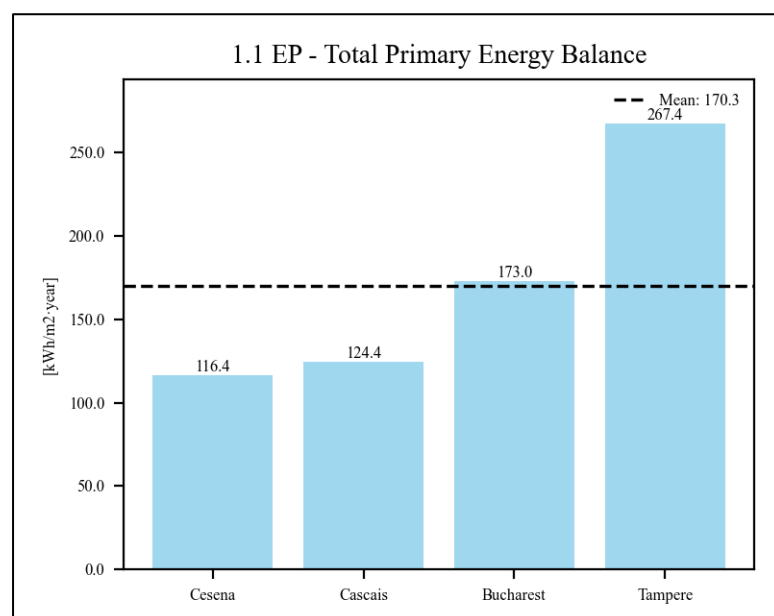
Figure 14. KPI 1.1 Total Primary Energy Balance compared for the 4 demo-sites.
